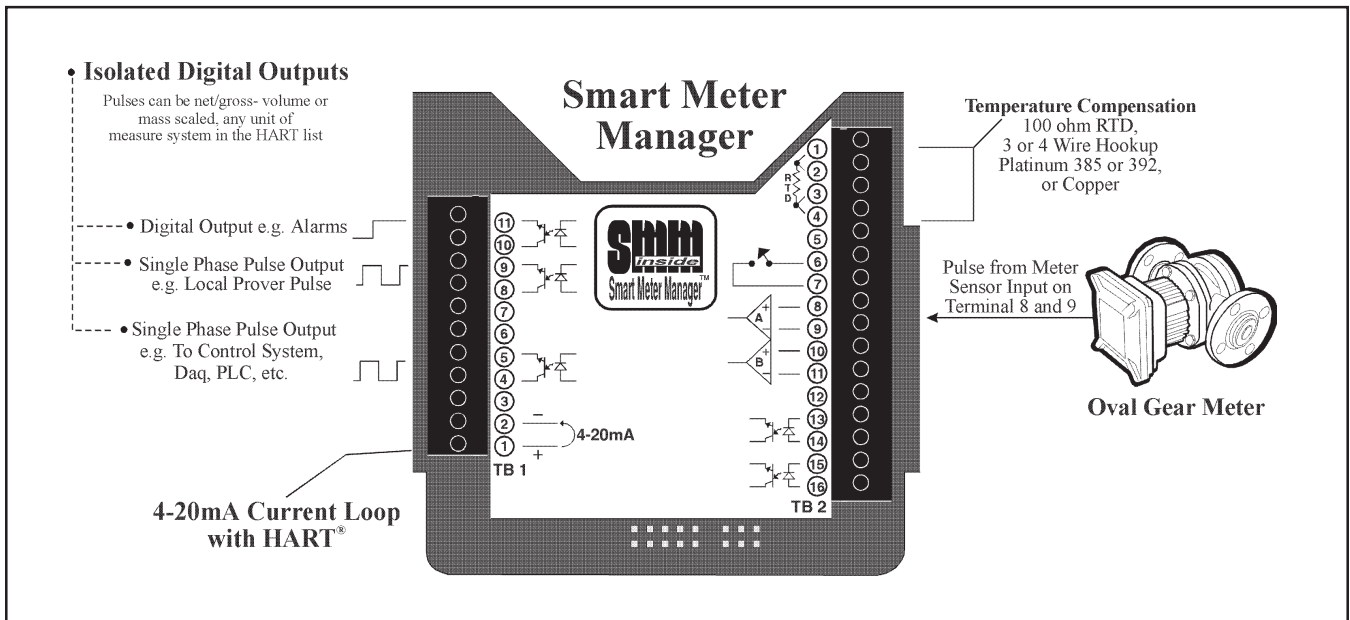
Figure 4 Typical Application: 9900 Series Oval Flowmeter with Smart Meter Manager™
