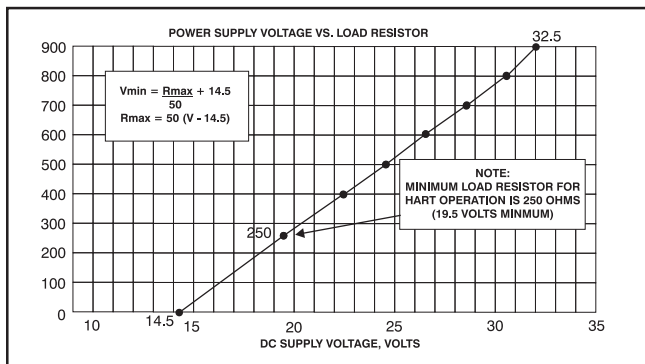
Figure 2 Maximum Load Resistance
