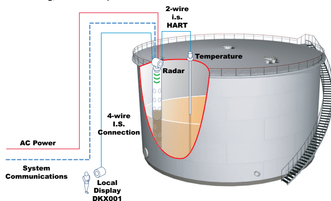
Example Tank Gauging System
